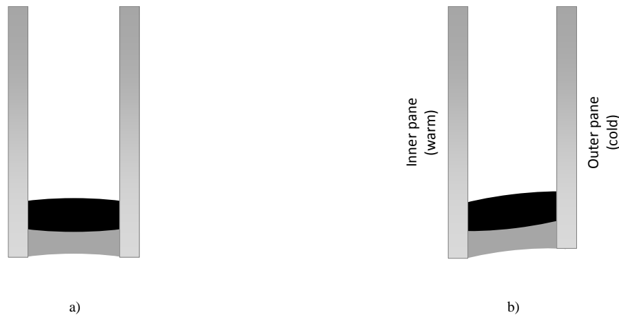
Fig. 19 Deformation of an IGU with Ködispace 4SG spacer, a) undeformed, b) deformed
