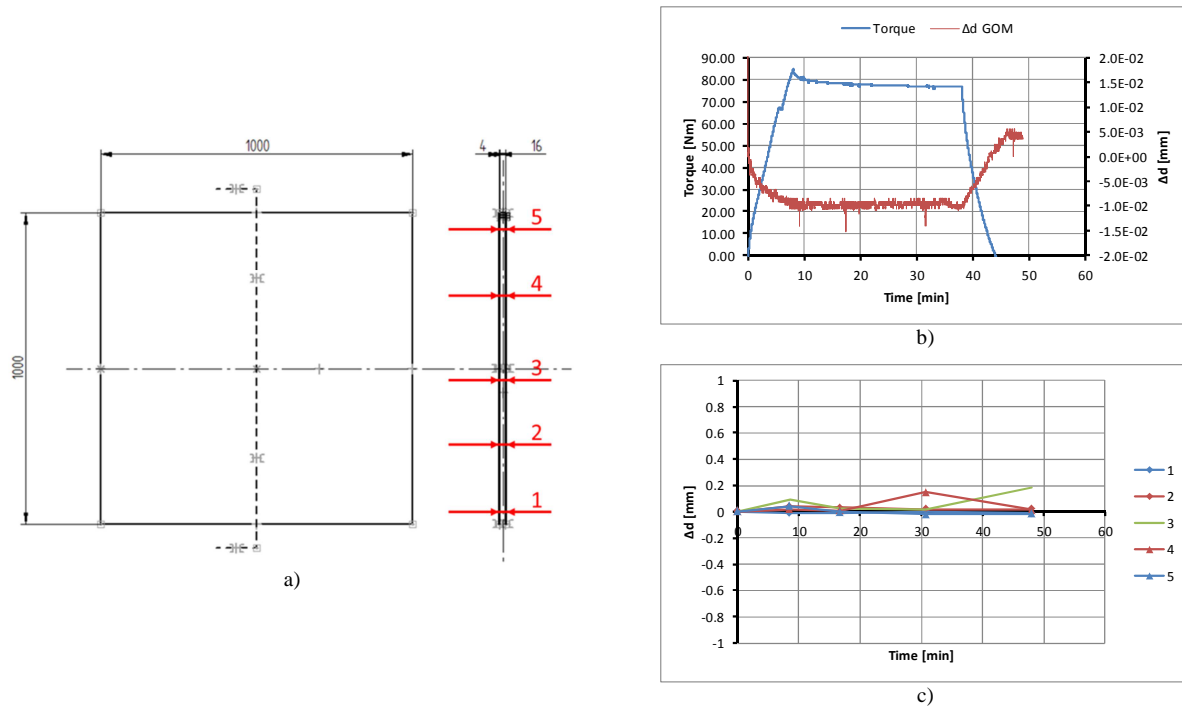
Fig. 21 Test results of the torsion test with IGUs \Delta l = 12 mm a) geometry and position of measuring point b) Torque and change of thickness over time (GOM System) c) Change in thickness over time measured with the micrometer
