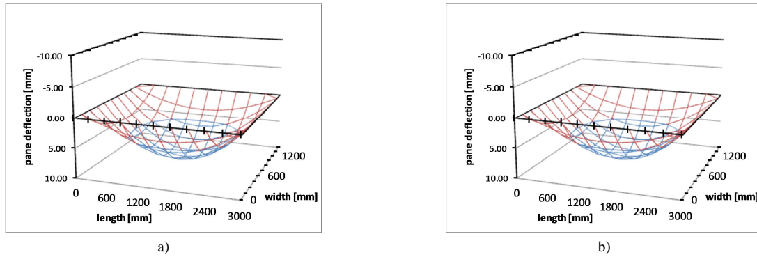
Fig. 13 Deflection of IGU glass panes (1500 x 3000 mm) with Ködispace 4SG spacer, a) ext. pane, b) int. pane
