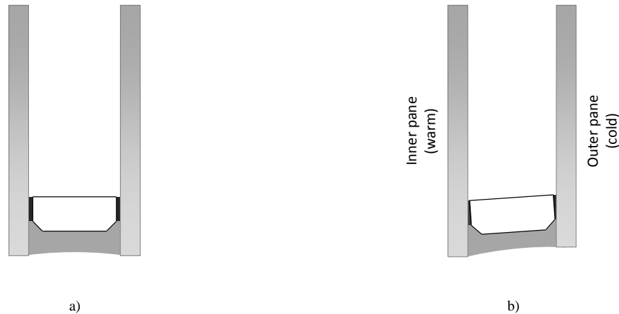
Fig. 18 Deformation of an IGU with conventional spacer due to thermal expansion, a) undeformed, b) deformed
