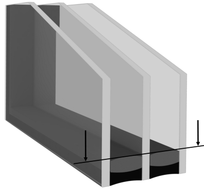
Fig. 4 Exact Alignment of the two frames with Ködispace 4SG
