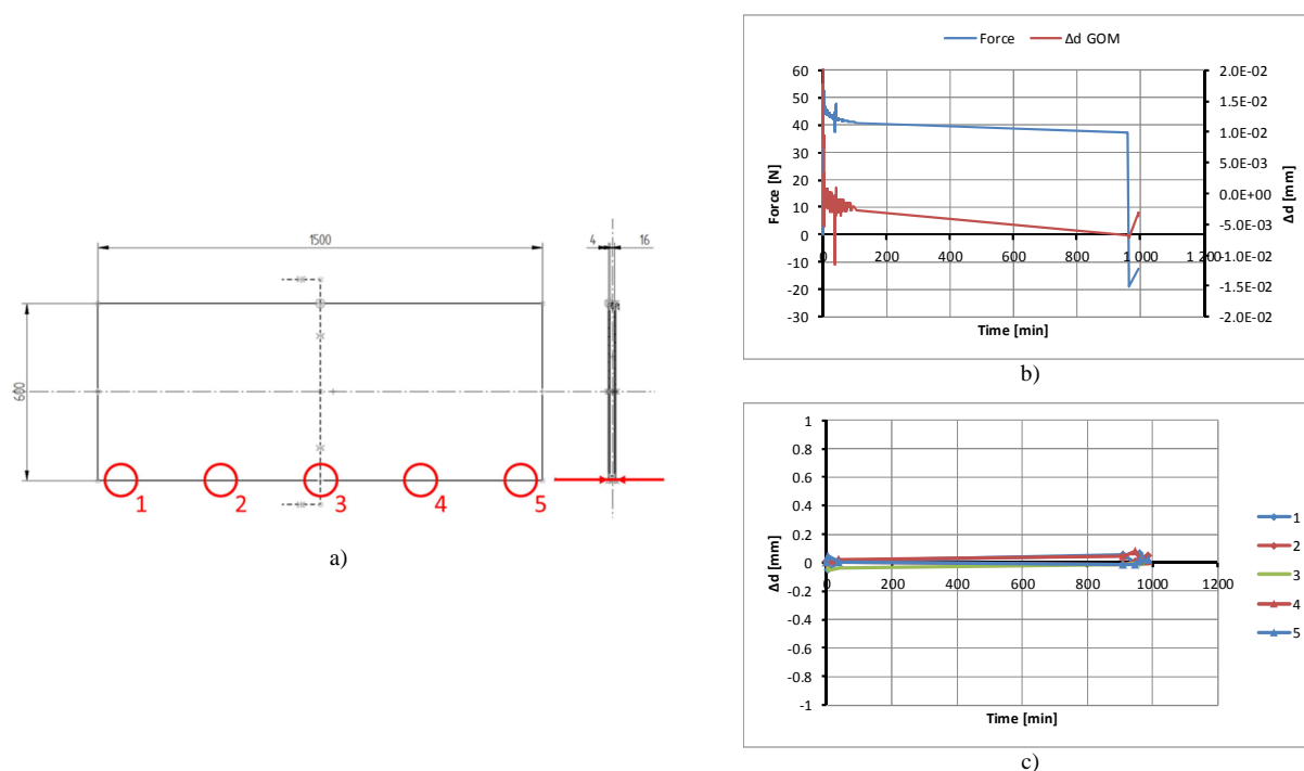
Fig. 23 Test results of the torsion test with IGUs \Delta l = 25 mm
