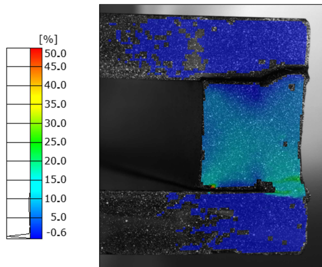
Fig. 17 Ködispace 4SG edge compound of an IGU model after applying a load in normal direction with stochastic pattern and derived major strain
