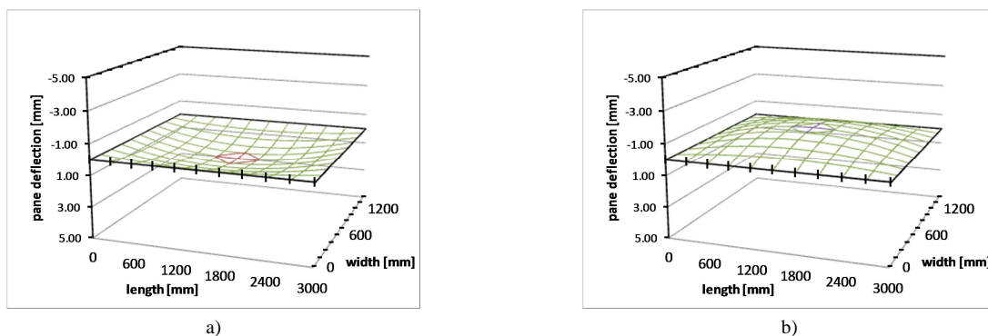
Fig. 11 Deflection of IGU glass panes ( 1500 \times 3000\text{ mm} ) with Ködispace 4SG spacer, a) ext. pane, b) int. pane
