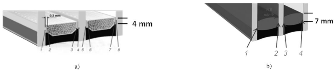
Fig. 27 Number of boundary layers and diffusion/permeation pathways a) conventional b) Ködispace 4SG
