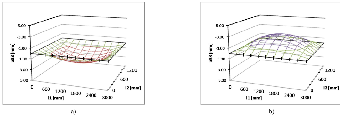
Fig. 10 Deflection of IGU glass panes ( 1500 \times 3000\text{ mm} ) with aluminum spacer, a) ext. pane, b) int. pane
